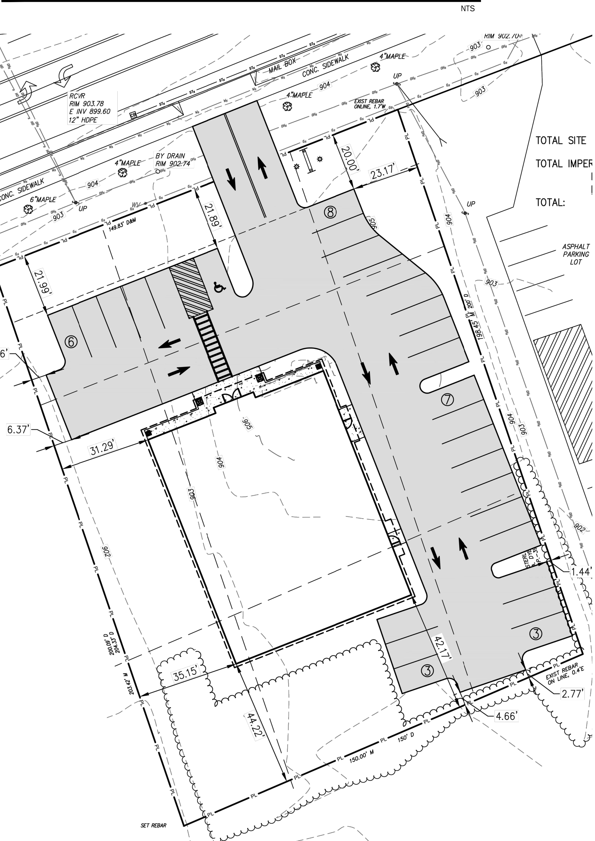
A1.2 Concept Site Plan
