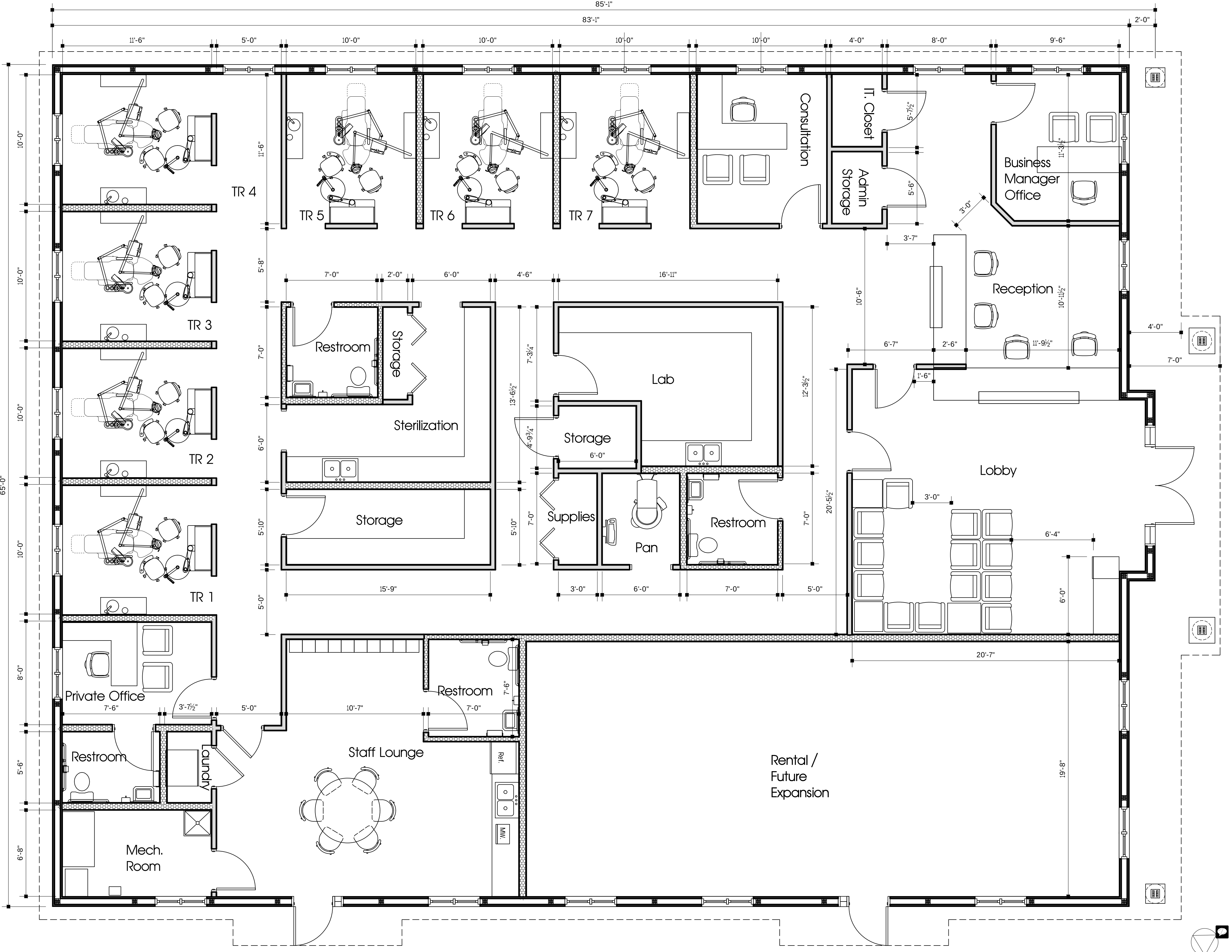
A1.3 Concept Floor Plan
